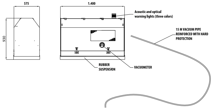
VACUUM UNIT INSTALLED BEHIND TO EXCAVATOR - WEIGHT: 600 kg
